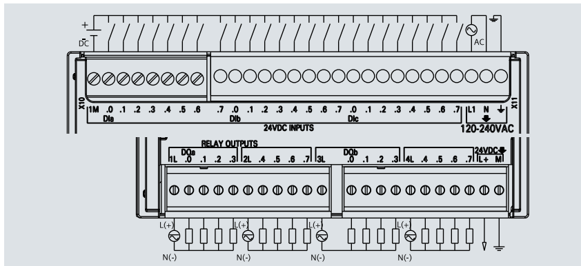
CPU SR40
