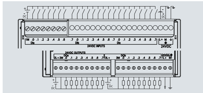
CPU ST40
